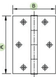
A=50 B=38 BRI95550X38 A=63 B=40 BRI95563X40 A=75 B=50 BRI95575X50 A=85 B=58 BRI95585X58
