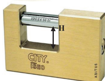
VIG4090197 L=90 H=36 VIG4090197KA UNIFICATI
