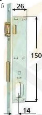
1 MAND+RULLO CIL. OVALE MG.913.14.2
