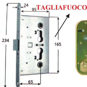
1 MAND.+SCROCCO FRONT. 24 Q9 MG.480.65.0
