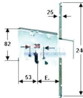
FASCIA E=70 CIL. EU CIS56013.70
